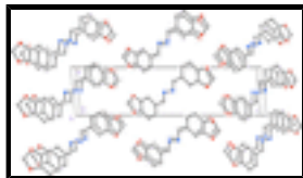
Fig. 2. Packing diagram of the title compound viewed along the b axis. The H atoms have been removed for clarity.
